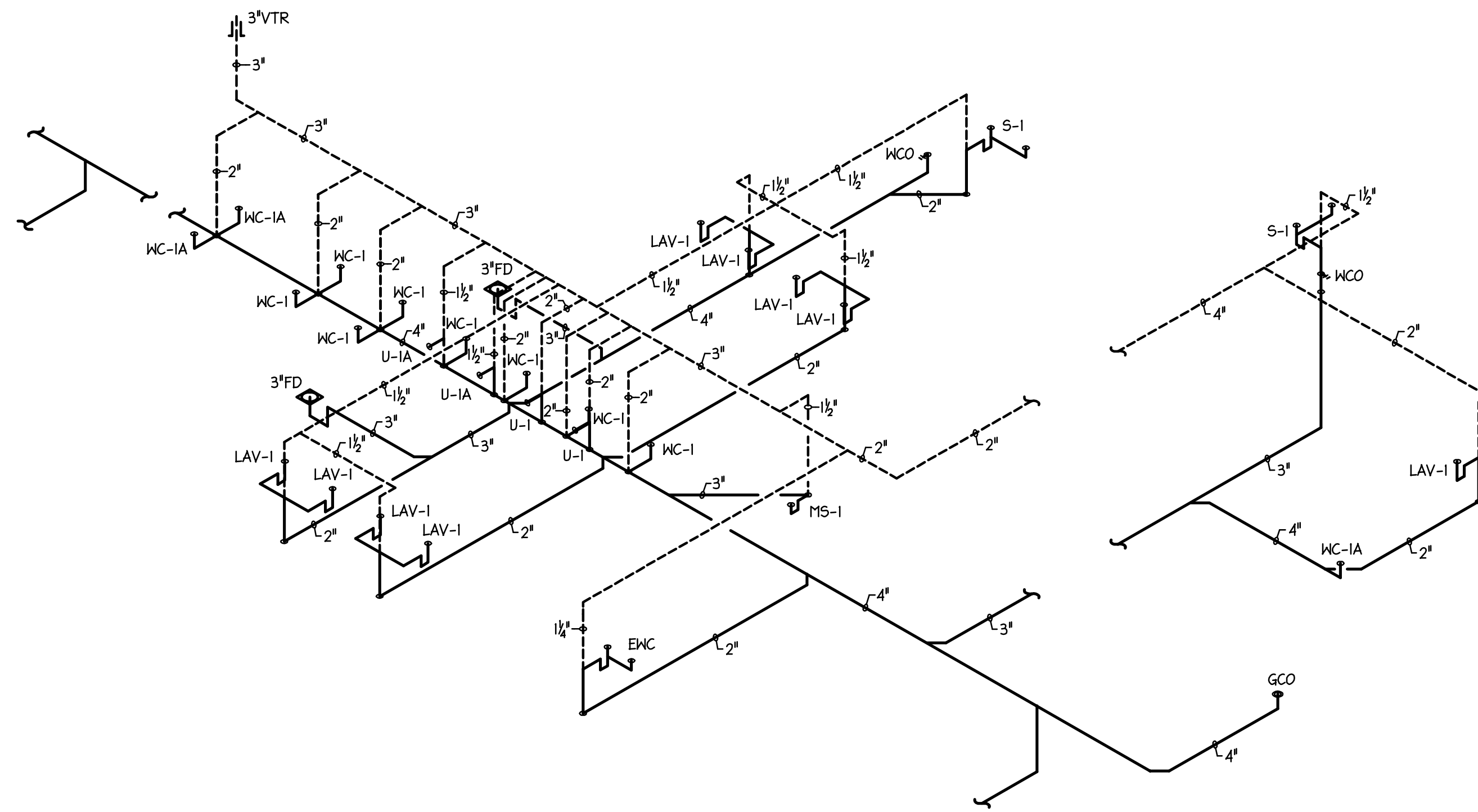
1 WASTE/VENT RISER DIAGRAM N.T.S.
