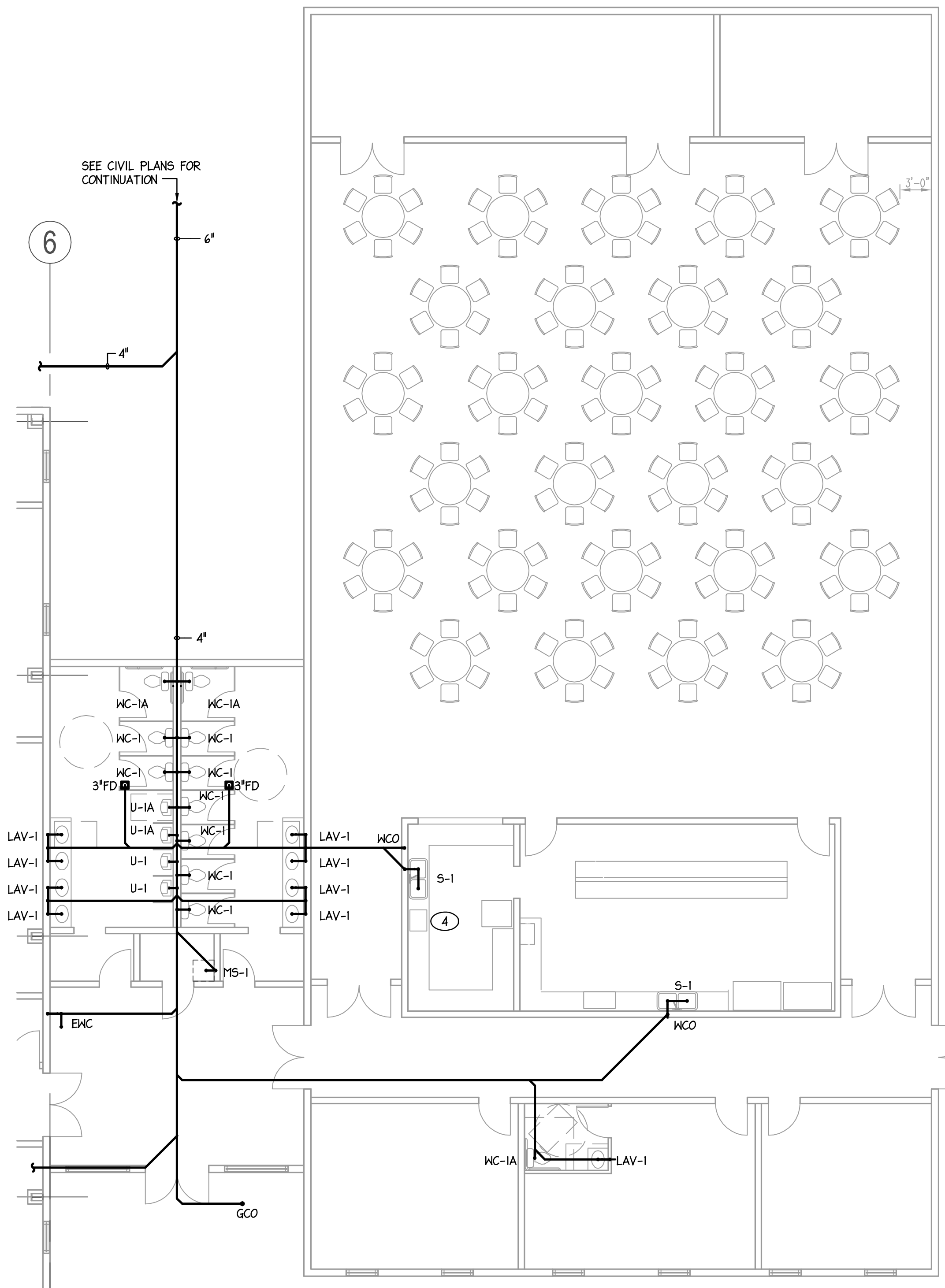
1 PLUMBING FELLOWSHIP HALL SANITARY PLAN 1/8" = 1'-0"
