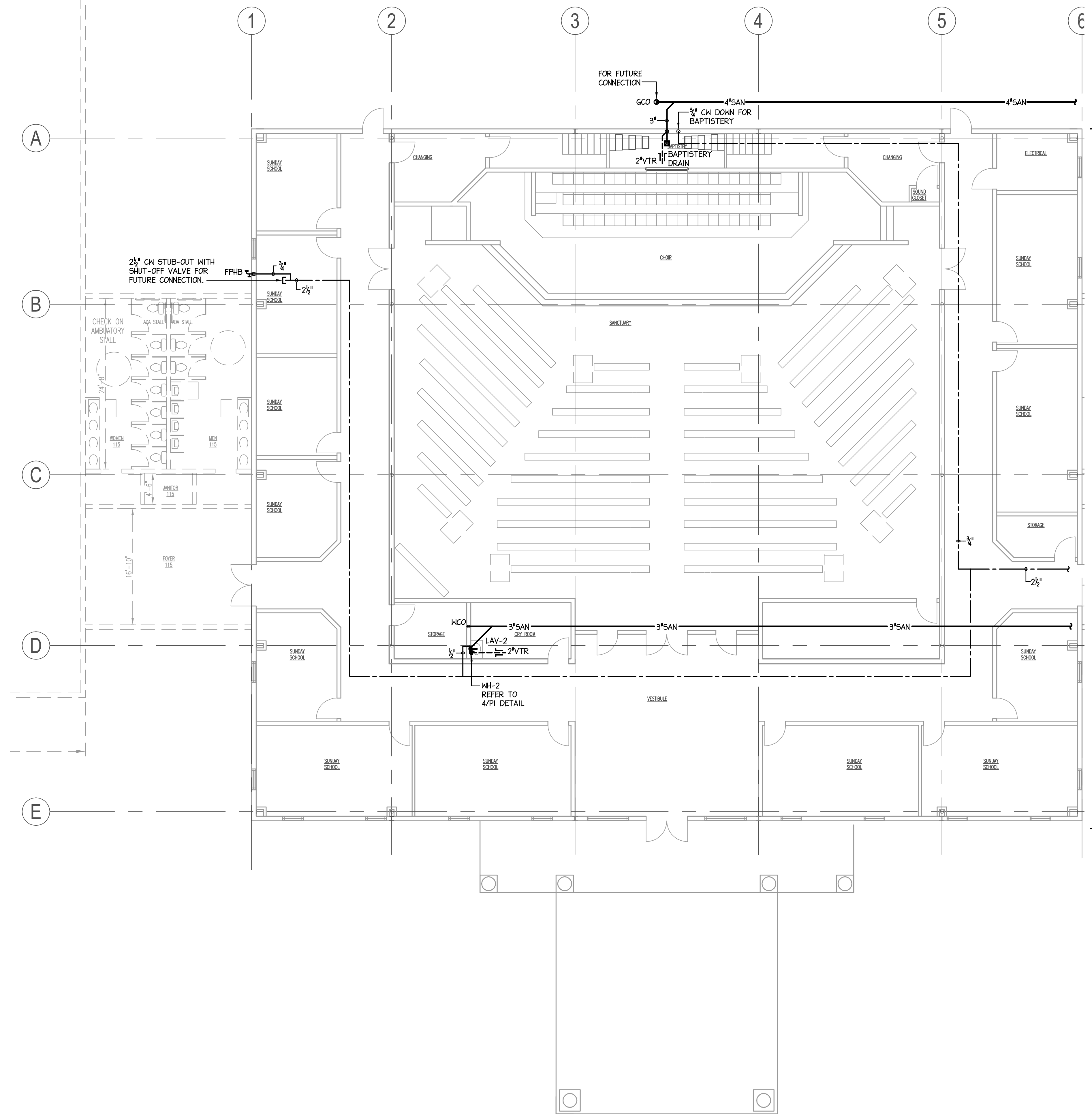
1 PLUMBING SANCTUARY PLAN 1/8" = 1'-0"
