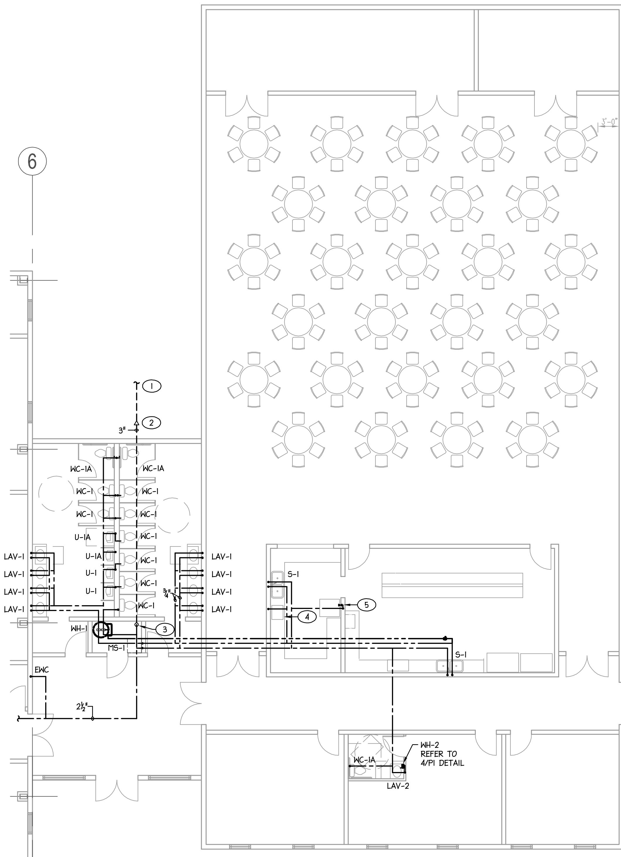
2 PLUMBING FELLOWSHIP HALL SUPPLY PLAN 1/8" = 1'-0"
