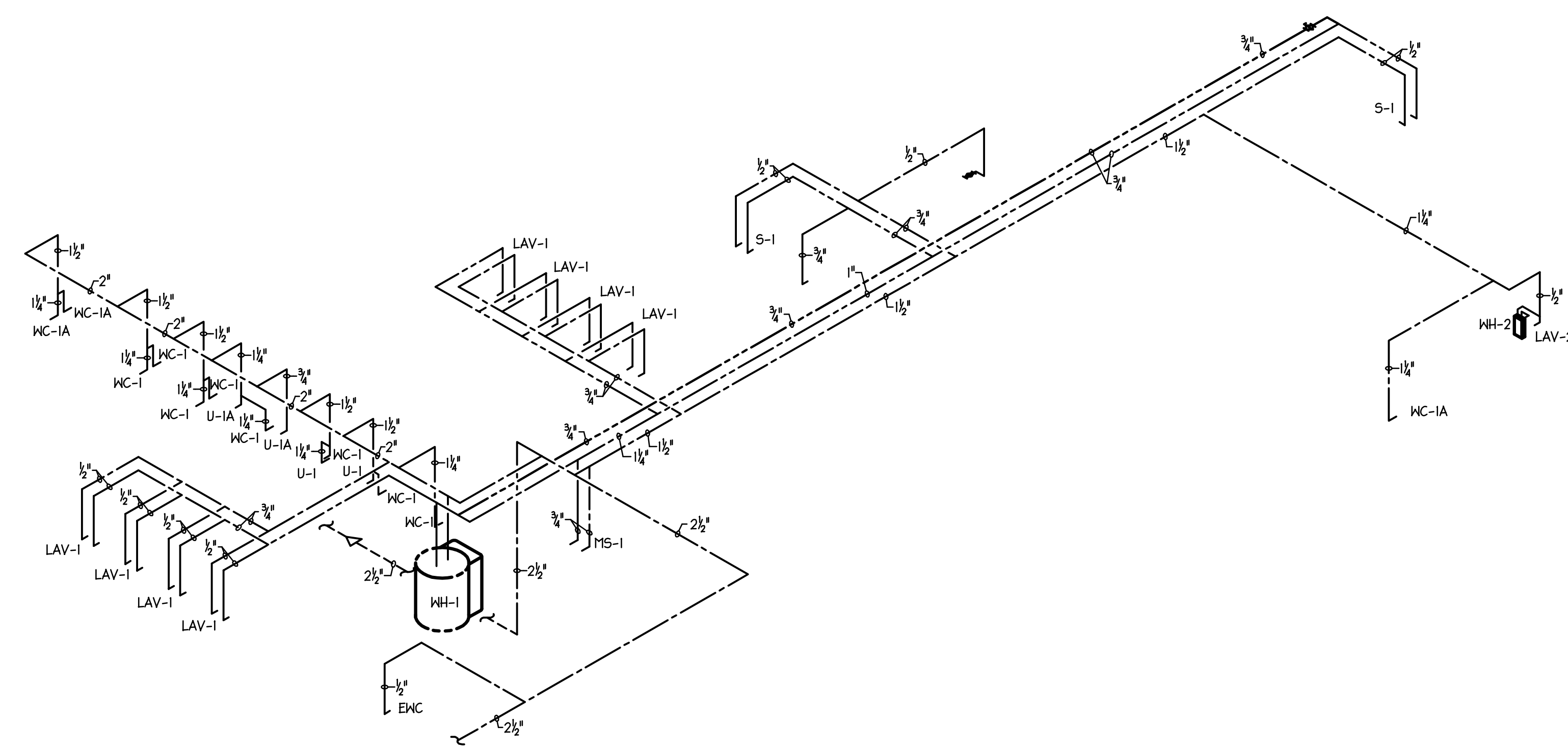
2 PLUMBING FELLOWSHIP HALL SUPPLY PLAN 1/8" = 1'-0"
